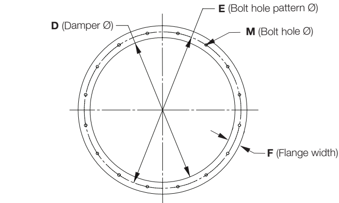
Round Flange Bolt Hole Pattern
