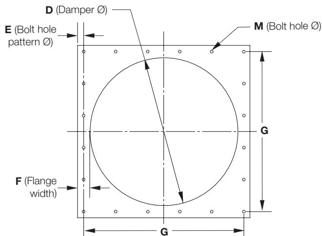
Square Flange Bolt Hole Pattern
