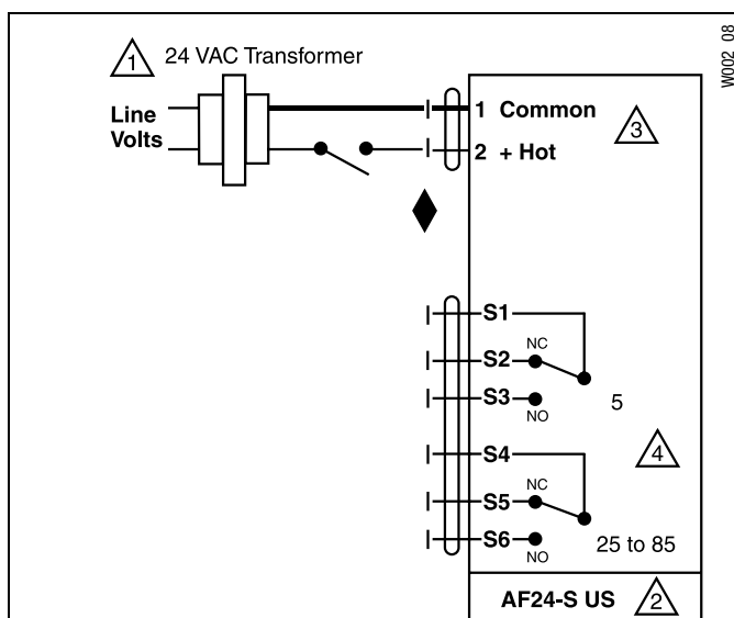
On/Off control for AF24-S US
