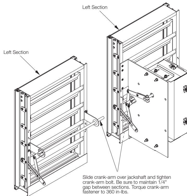
Multi-Section Installation
