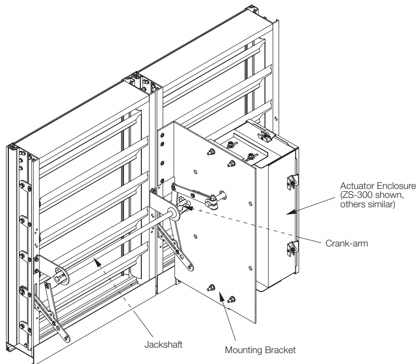
Multi-Section Configuration
