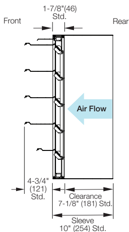
Vertical Mount with Sleeve (discharge)
