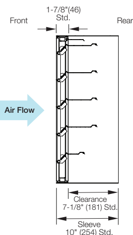
Vertical Mount with Sleeve (intake)
