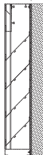
2" Insulated (8.75 R-value)
