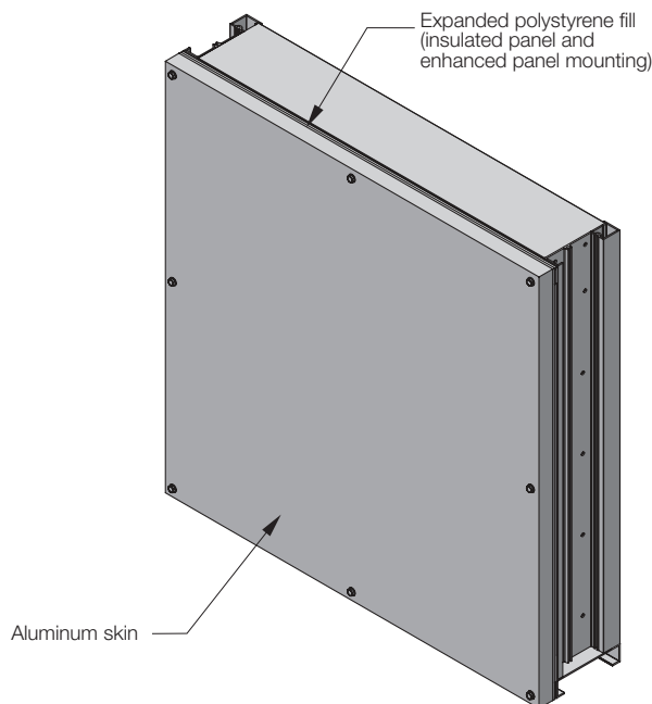
Building Interior View
