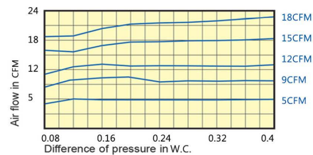
eFlow-CAR LOW Pressure(LP) 4"/5" 18 - 35CFM
