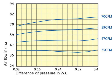
eFlow-CAR LOW Pressure(LP) 5" 35 - 70CFM
