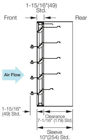
Vertical Mount with Sleeve (intake)
