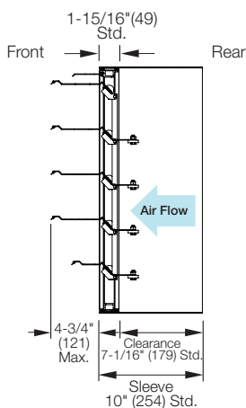
Vertical Mount with Sleeve (discharge)
