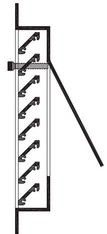
Flap Blade Damper (Optional)
