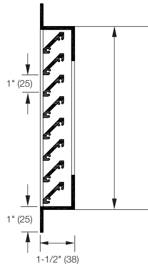
Vertical Section (Standard)
