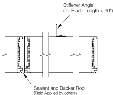
Vertical Section †Screen adds approximately 3/16" (5) to louver depth
