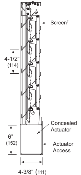
Vertical Section
