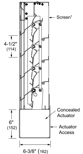
Vertical Section
