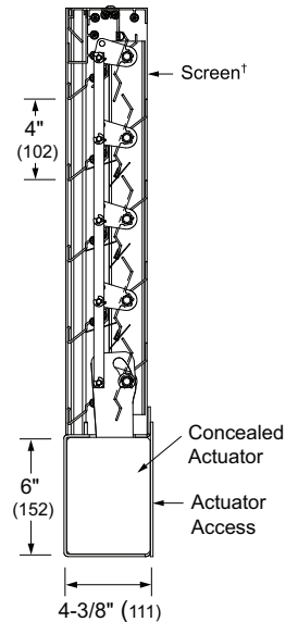
Vertical Section
