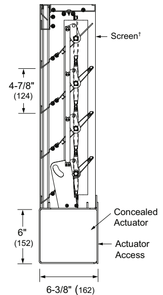
Vertical Section
