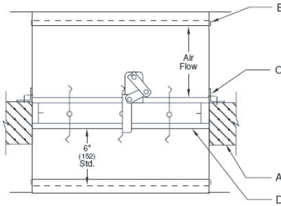
Horizontal Mount (Single Side Mounting Angle)
