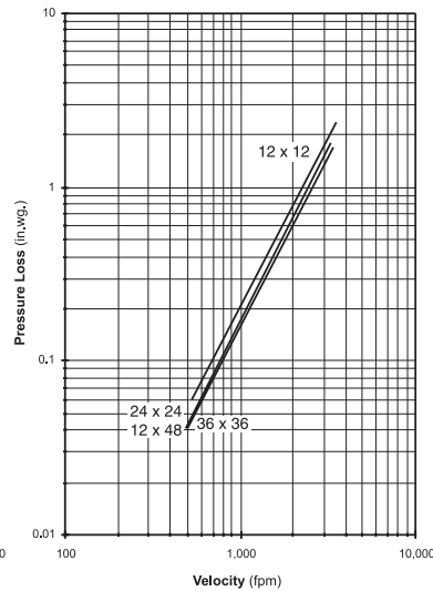
Figure 5.5 — Plenum Mount
