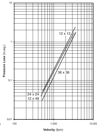
Figure 5.2 — Ducted Inlet
