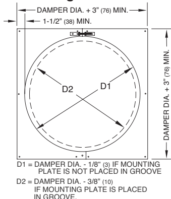
Figure 6 - Mounting Plate
