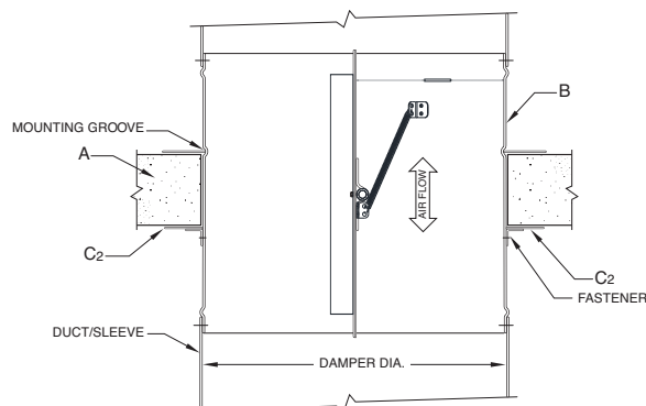
Figure 1a Horizontal Concrete Partition
