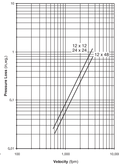
Figure 5.2 — Ducted Inlet
