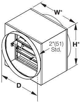
Sleeve Style AR (Optional) Round duct transitions are standard with D=W=H . (available with D<W and H )
