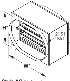
Style AO (Optional) Oval duct transitions are standard with W and H equal to damper width and height dimensions. (available with W and H smaller than damper width and height)
