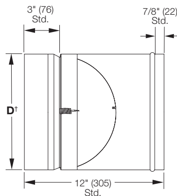
Side View (Integral Sleeve)
