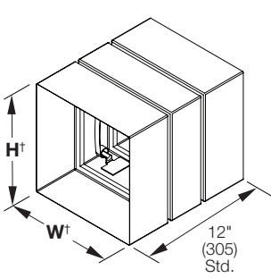
Sleeve Style ISA (Optional)
