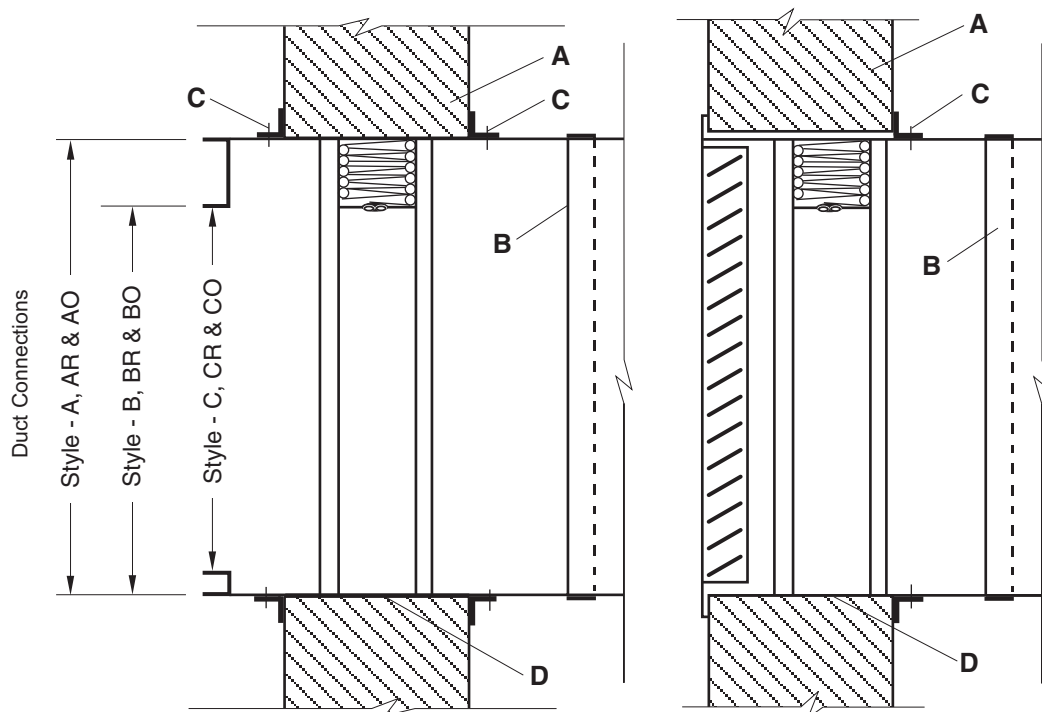
Damper Installation For Typical Fire Rated Partition
