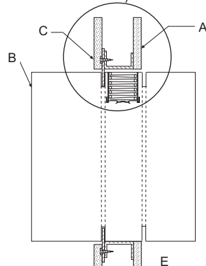
FIGURE 3: Metal Stud Angle UNDER Drywall
