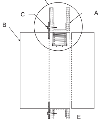
FIGURE 2: Metal Stud Angle Over Drywall
