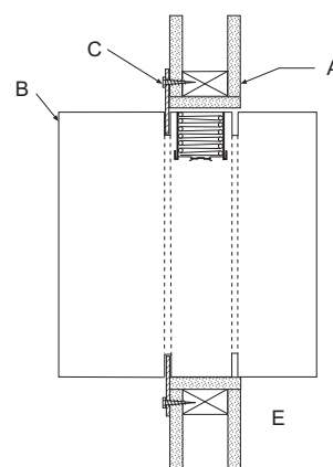
FIGURE 4: Wood Stud
