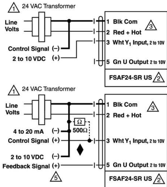
Proportional control
