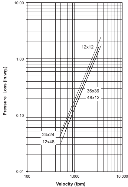
Figure 5.2 — Ducted Inlet
