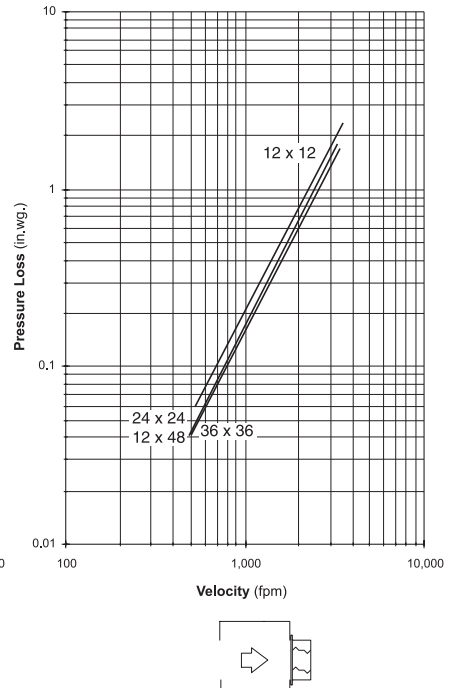
Figure 5.5 — Plenum Mount
