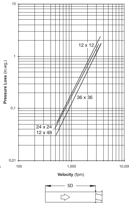
Figure 5.2 — Ducted Inlet
