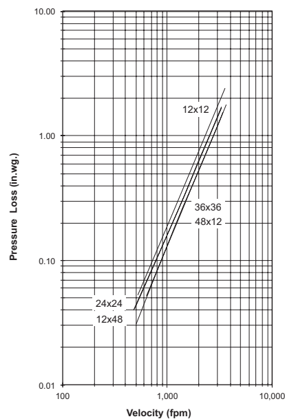
Figure 5.2 — Ducted Inlet
