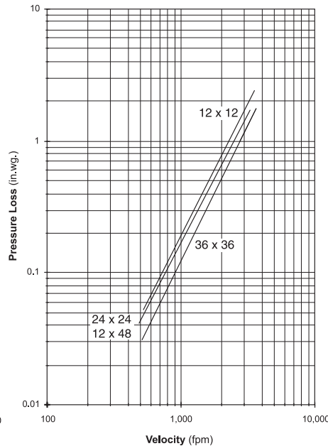
Figure 5.2 — Ducted Inlet
