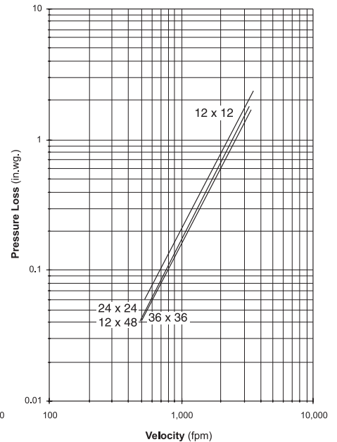
Figure 5.5 — Plenum Mount
