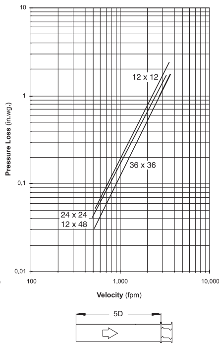
Figure 5.2 — Ducted Inlet
