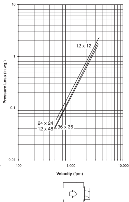
Figure 5.5 — Plenum Mount
