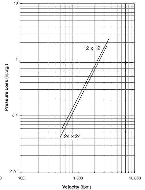
Figure 5.5 — Plenum Mount
