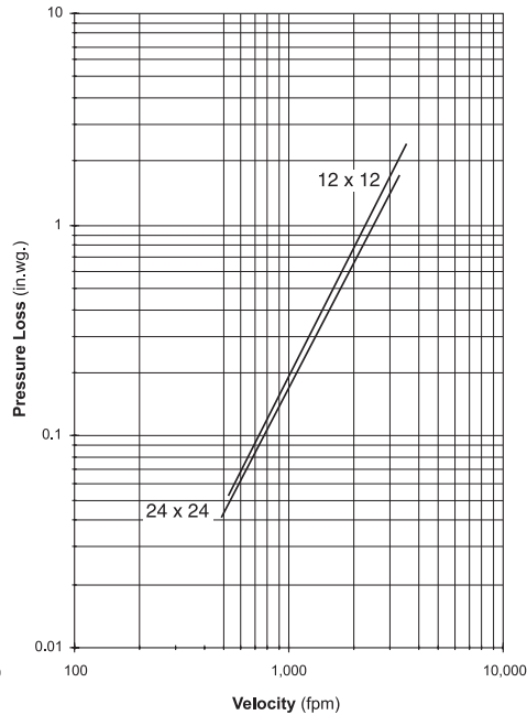
Figure 5.2 — Ducted Inlet
