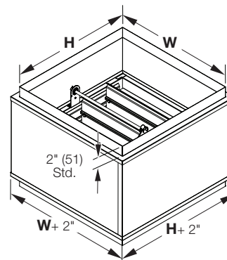
Type C (Optional) Damper is oversized and uses rectangular transitions to remove damper frame from airstream
