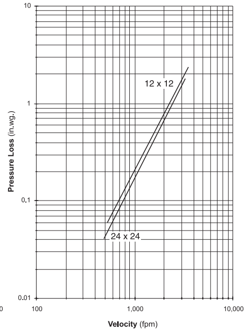
Figure 5.5 — Plenum Mount
