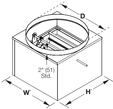
Type R (Optional) Round duct transitions are standard with D=W=H . (available with D<W and H )
