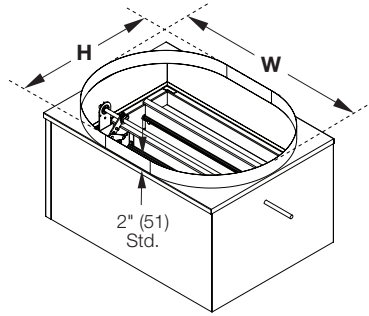
Type O (Optional) Oval duct transitions are standard with W and H equal to damper width and height dimensions. (available with W and H smaller than damper width and height)
