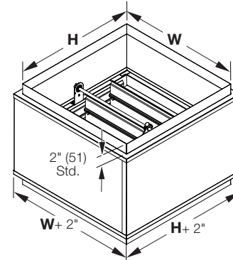
Type C (Optional) Damper is oversized and uses rectangular transitions to remove damper frame from airstream
