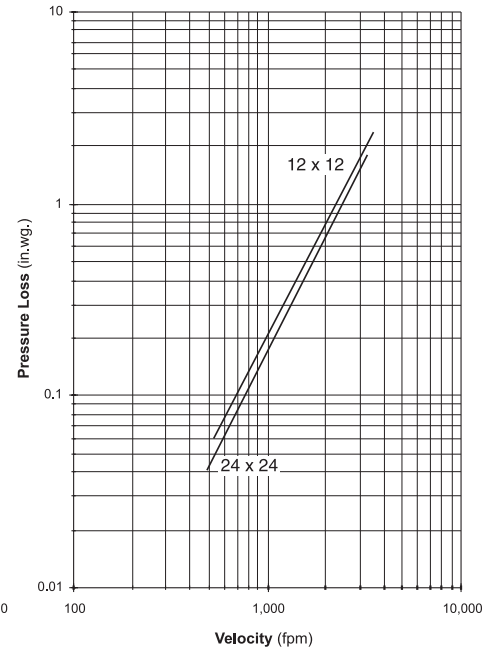
Figure 5.5 — Plenum Mount
