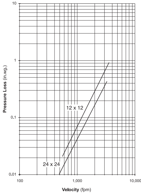
Figure 5.3 — Ducted Inlet and Outlet
