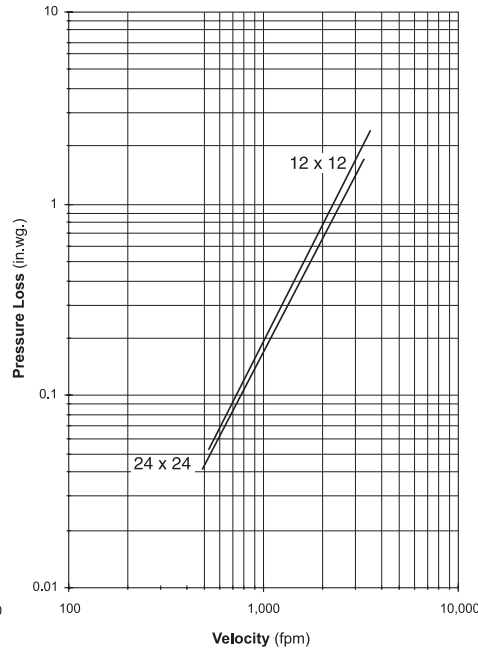
Figure 5.2 — Ducted Inlet
