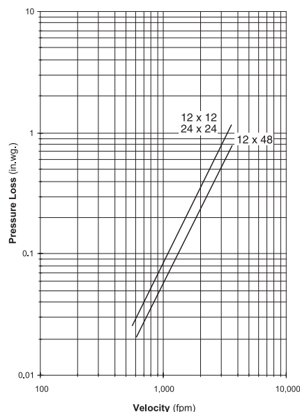
Figure 5.2 — Ducted Inlet
