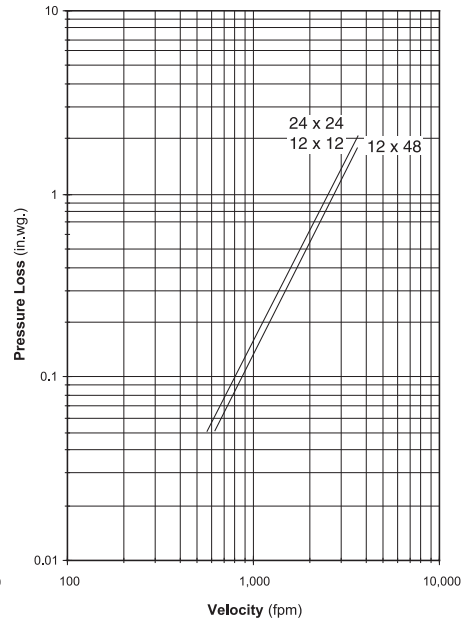
Figure 5.5 — Plenum Mount
