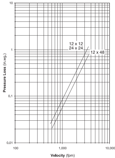
Figure 5.2 — Ducted Inlet
