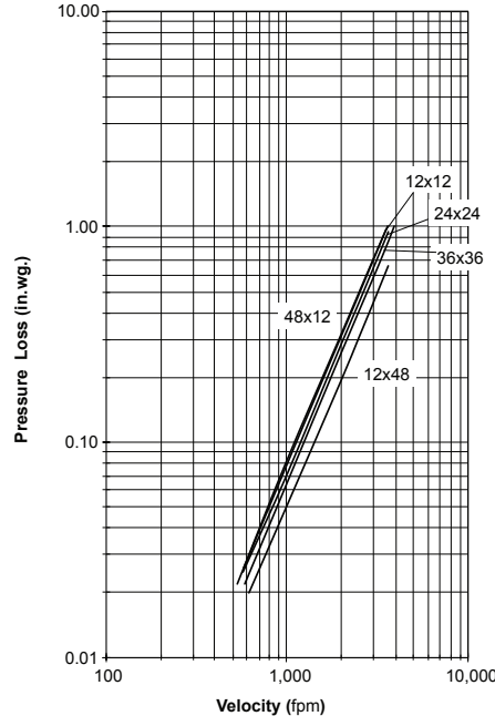
Figure 5.2 — Ducted Inlet
