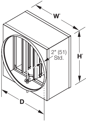
Type R (Optional) Round duct transitions are standard with D=W=H . (available with D<W and H )
