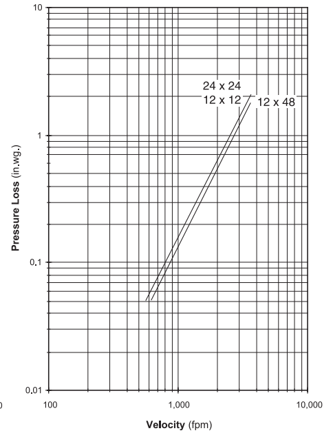
Figure 5.5 — Plenum Mount
