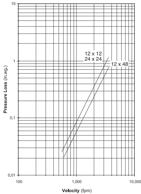
Figure 5.2 — Ducted Inlet
