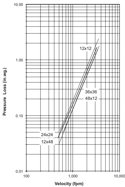
Figure 5.2 — Ducted Inlet
