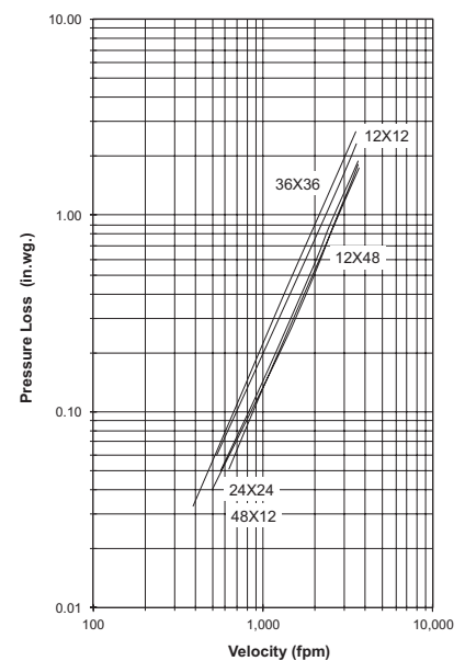
Figure 5.5 — Plenum Mount
