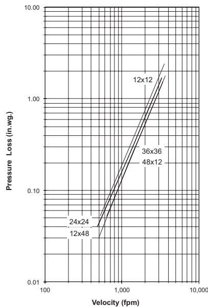
Figure 5.2 — Ducted Inlet
