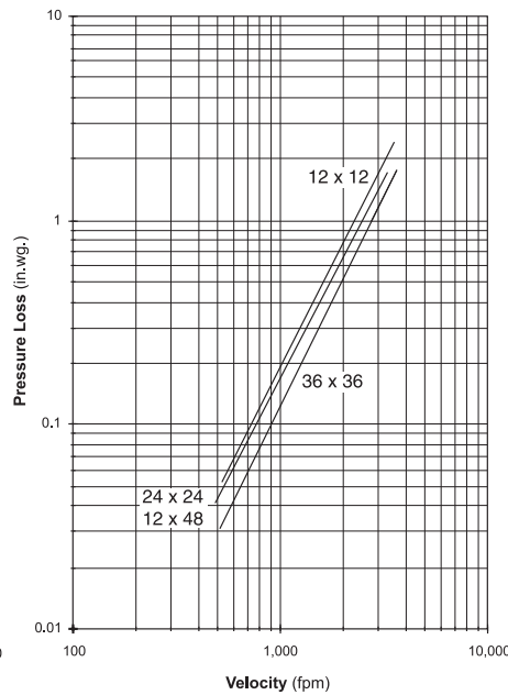
Figure 5.2 — Ducted Inlet
