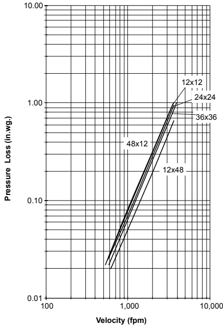
Figure 5.2 — Ducted Inlet
