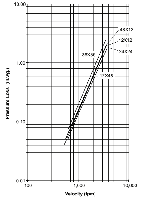
Figure 5.5 — Plenum Mount
