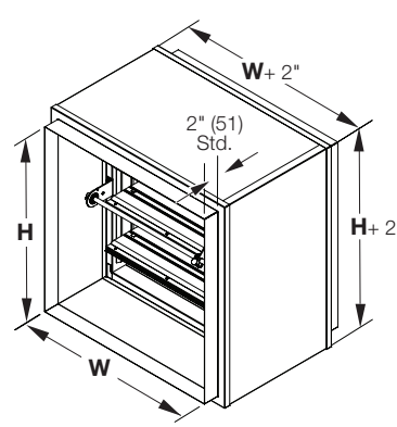
Type C (Optional) Damper is oversized and uses rectangular transitions to remove damper frame from airstream
