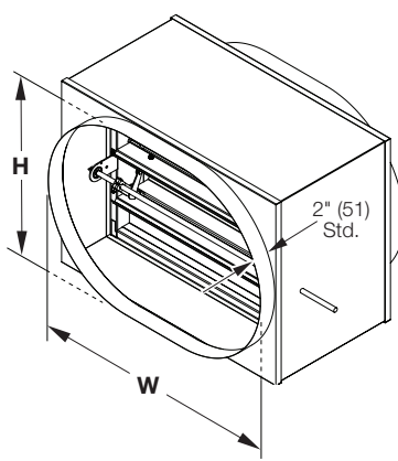
Type O (Optional) Oval duct transitions are standard with W and H equal to damper width and height dimensions. (available with W and H smaller than damper width and height)
