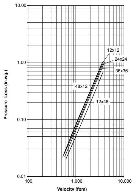
Figure 5.2 — Ducted Inlet
