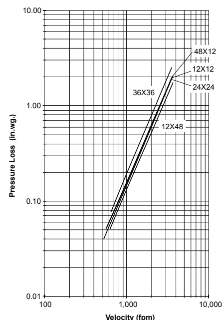
Figure 5.5 — Plenum Mount
