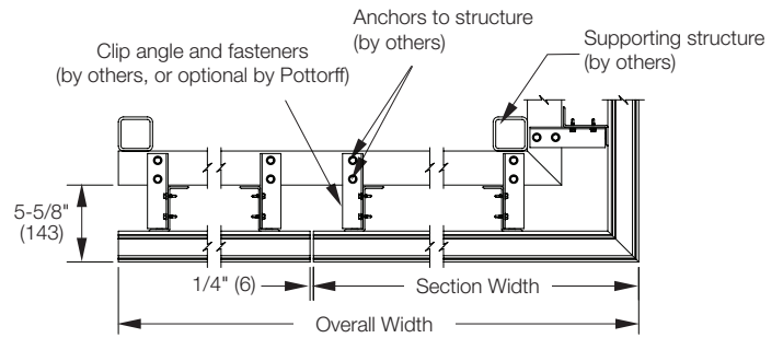
Generic Plan View - Outside Mitered Corner
