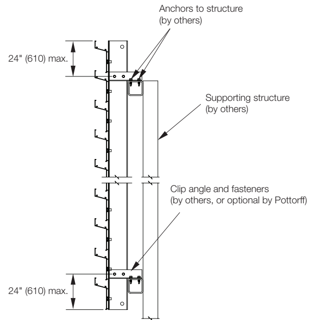
Vertical Section
