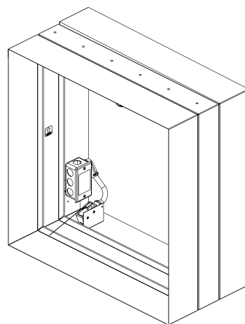
Model PI-10 (sleeve option), internal mount wiring box
