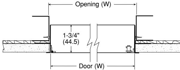
Model PW Typical Wall Installation
