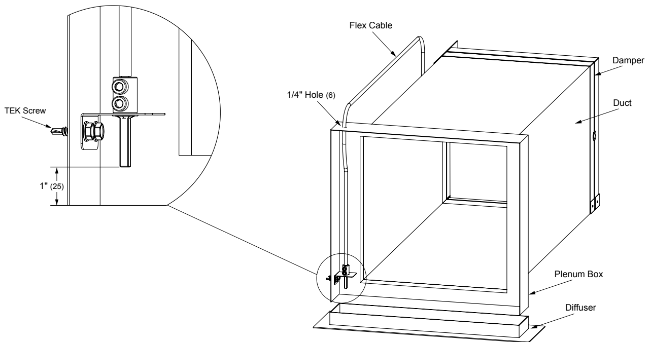
Figure 3 Final Installation
