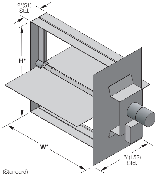
RD-10 (Standard) *Damper dimensions furnished approximately 1/8" (3) undersize
