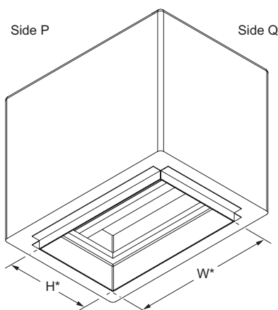
Model RD-521-IP (standard) *Damper dimensions furnished approximately net O.D.
