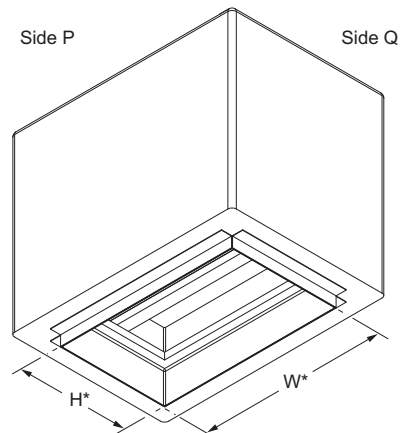
Model RD-521-IP-G (standard) *Damper dimensions furnished approximately net O.D.
