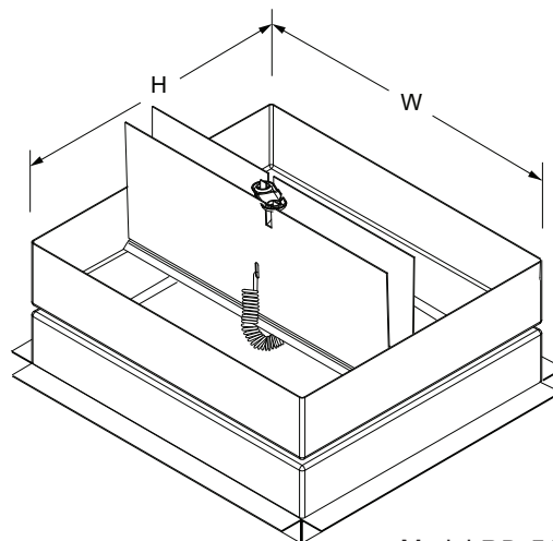
Model RD-521-NP-G (standard) *Damper dimensions furnished approximately net O.D.
