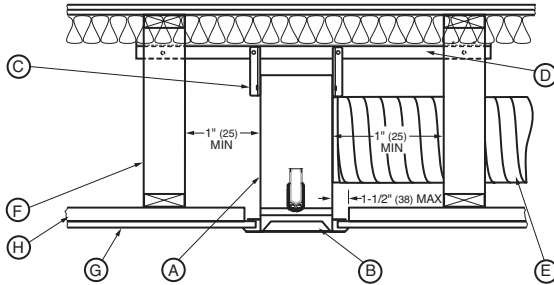
END VIEW - Duct to Grille Connection
